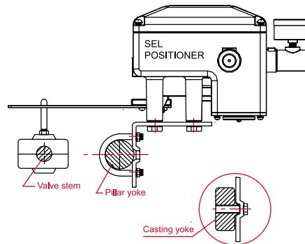
Mounting to Linear Actuator to IEC 534
