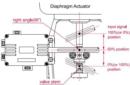
Feedback Lever Installation
